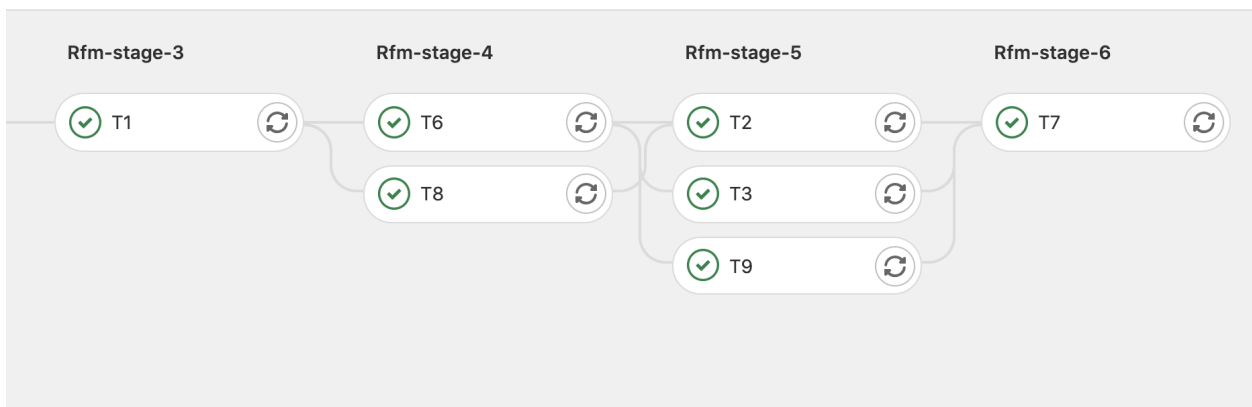
Fig. 5: Snapshot of a Gitlab pipeline generated automatically by ReFrame.
